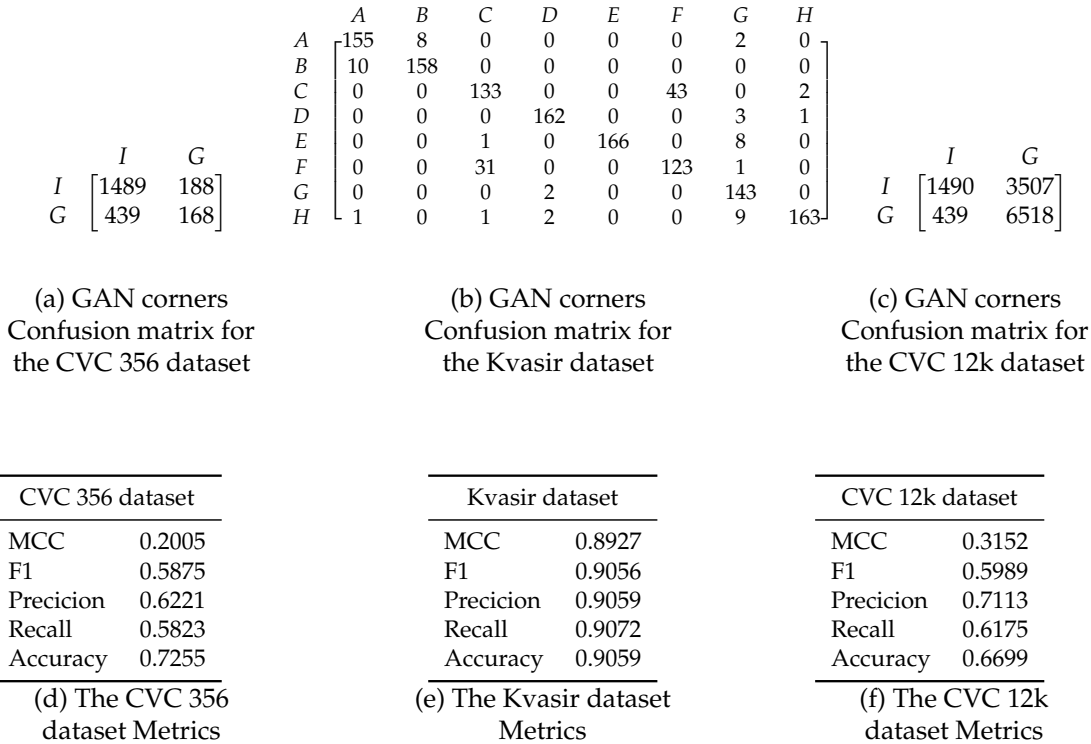
Figure 4.24: InceptionResNetV2 Inpainted corners with the GAN results
