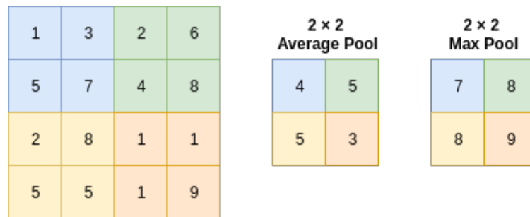
Figure 2.12: Both max and average pooling done on a 4 \times 4 matrix
