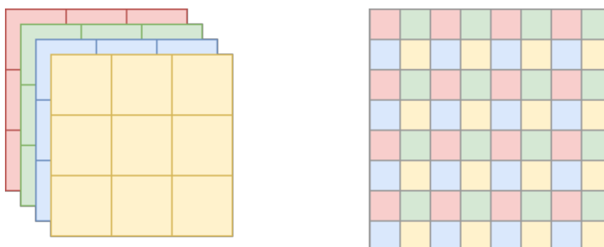
Figure 3.9: How the layers in the sub pixel layer is stacked. Recreated from the SubPixel paper by Shi et al. [76]
