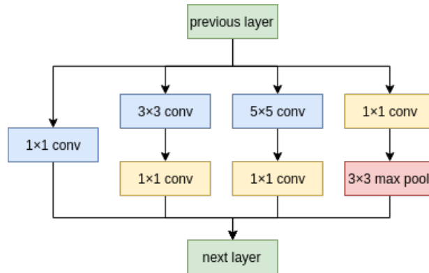
(b) Inception module concept as proposed in [61]
