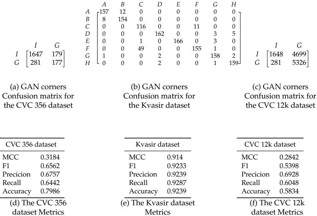
Figure 4.17: Densenet121 Inpainted corners with the GAN results
