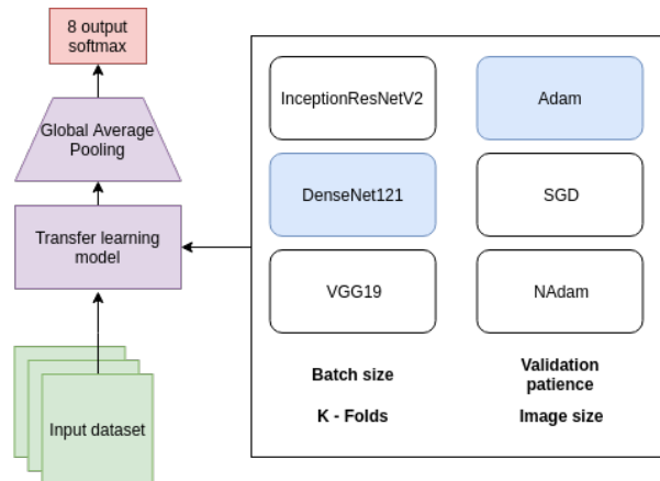
Figure 3.5: The model we use for classifying with the most important options for the learning process.
