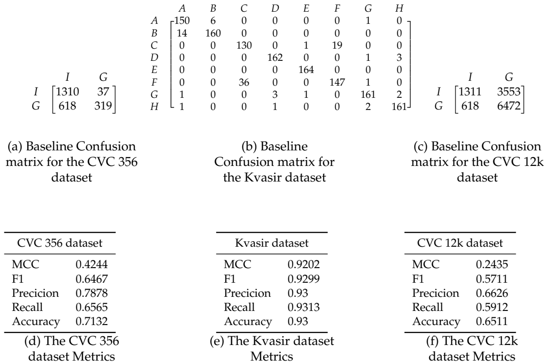
Figure 4.16: Densenet121 Base results
