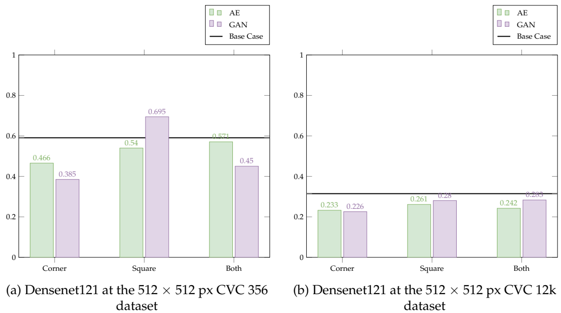
Figure 4.33: Visualisation of two out of the three datasets with Densenet121 at 512 × 512 px
