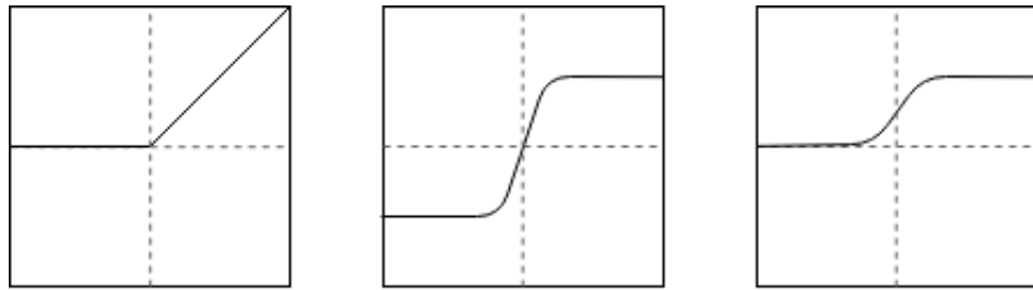
Figure 2.11: Activation functions from -2 to 2 on each axis. From left to right: ReLu, Tanh, Sigmoid
