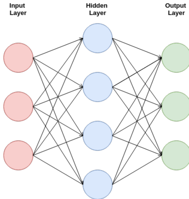
Figure 2.9: Simple illustration of a multilayer perceptron with three inputs, one hidden layer with four nodes, and one output layer with three nodes.
