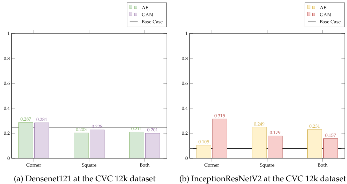
Figure 4.32: Visualisation of the CVC 12k MCC values made by both Densenet121 and InceptionresnetV2
