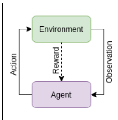
Figure 2.5: The basic structure of reinforcement learning
