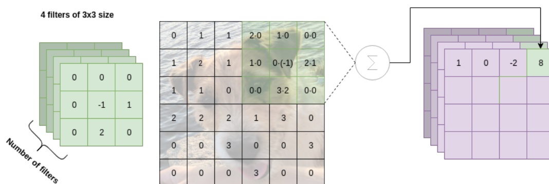
Figure 2.10: The values calculated when a convolutional filter after 4 sliding window operations, here the number of inputs does not represent how many inputs there usually is in an image
