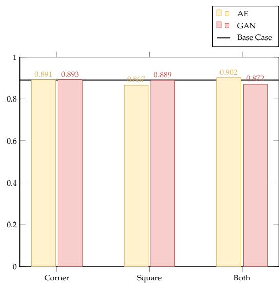
(b) InceptionResNetV2 at the Kvasir dataset
