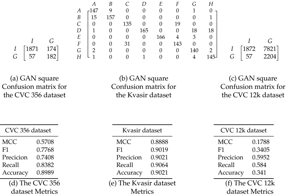
Figure 4.26: InceptionResNetV2 Inpainted square with the GAN results
