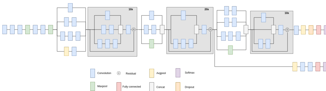
Figure 3.7: The compressed view of the InceptionResNetV2 network inspired by Mahdianpari et al.
