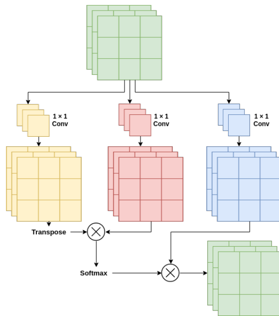
Figure 3.10: How the layers in the Self-Attention layer is stacked. Recreated from the Self-Attention paper by Zhang et al. [77]
