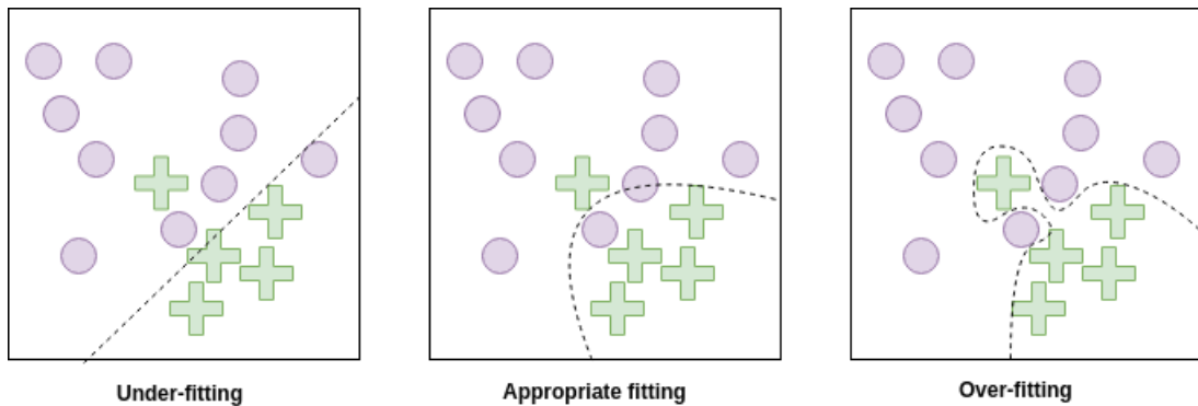
Figure 2.14: Three cases of data boundary prediction. In most cases we desire appropriate amount of fitting to our dataset to keep generalisation
