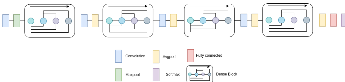
Figure 3.8: The compressed view of the DenseNet network inspired by Mahdianpari et al.
