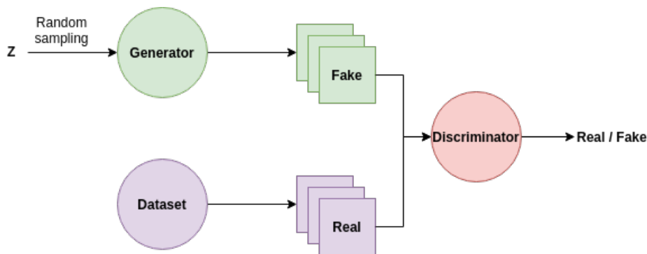
Figure 2.17: The basic concept of the generative adversarial network
