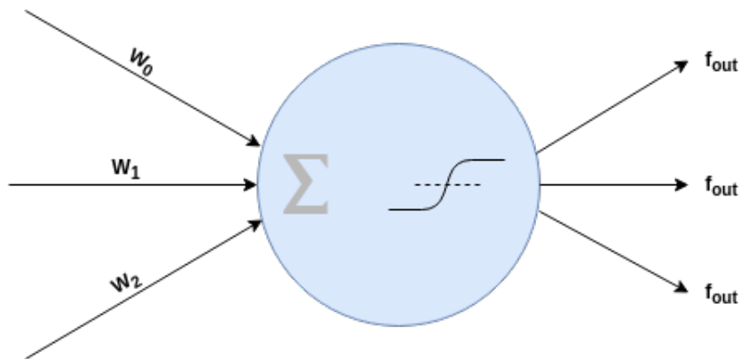
Figure 2.8: Simple perceptron that sends out an output that is the tanh of the the sum of the inputs
